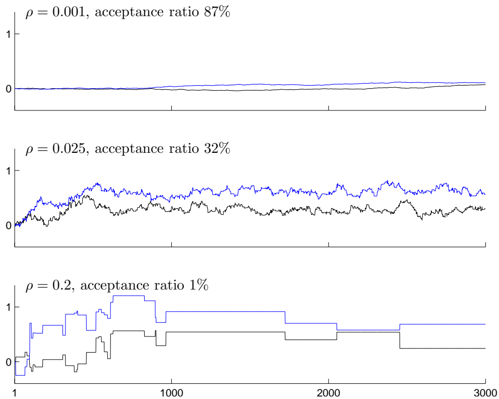
Figure 5.3: Three different choices of proposal distribution in Metropolis-Hastings algorithm: \rho = 0.001 , \rho = 0.025 and \rho = 0.2 in formula (5.16). Plotted are components 8 (black line) and 16 (blue line) of the sample vectors. In the top plot \rho is too small and the chain moves very slowly. In the middle plot \rho is quite appropriate, whereas in the bottom plot \rho is too large, leading to the rejection of most candidates.
